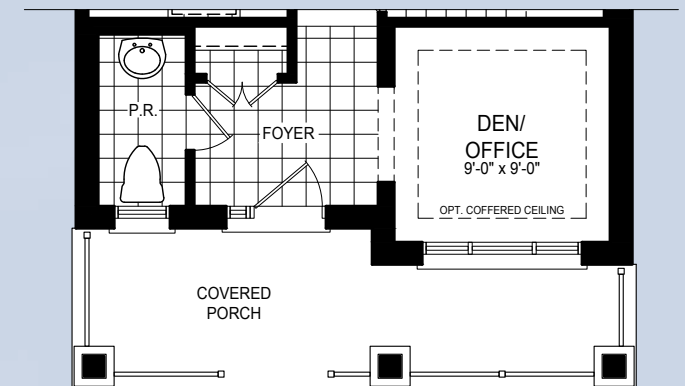
Ground Floor Elevation B
